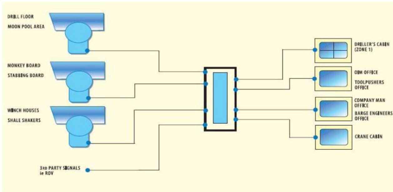
Typical Driller's TV System
